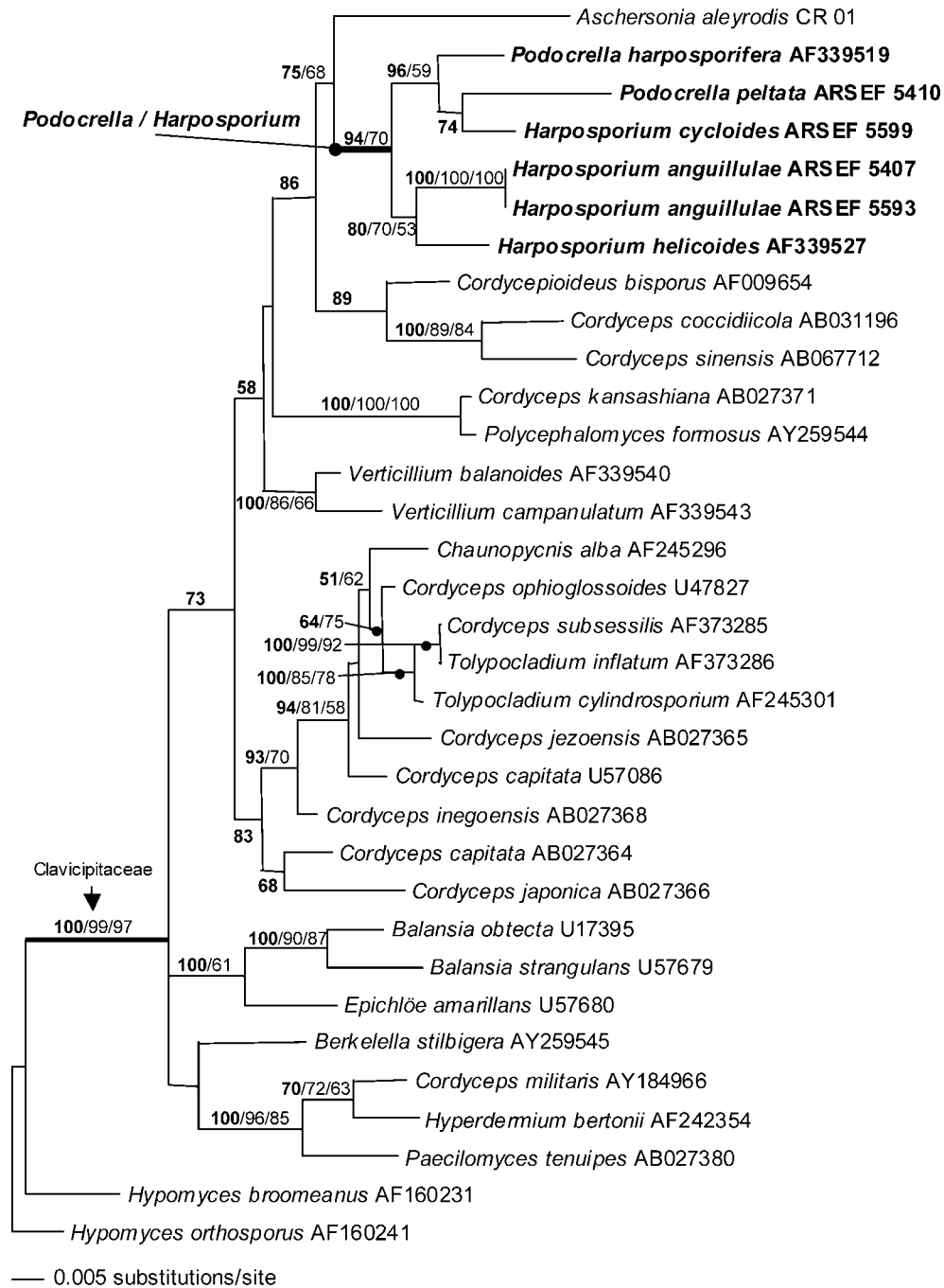
FIG. 1. LSU cladogram with the best log-likelihood (-3320.83) obtained in the Bayesian analysis. Numbers at nodes indicate values for posterior probability (%) in Bayesian analysis (bold)/neighbor-joining bootstrap/maximum parsimony bootstrap. Maximum parsimony (MP) analysis scores: 645 characters are constant, 40 characters are parsimony uninformative, 115 characters are parsimony informative (14.4%), 3 MP trees, 419 steps, CI: 0.47, RI: 0.62, HI: 0.53.
